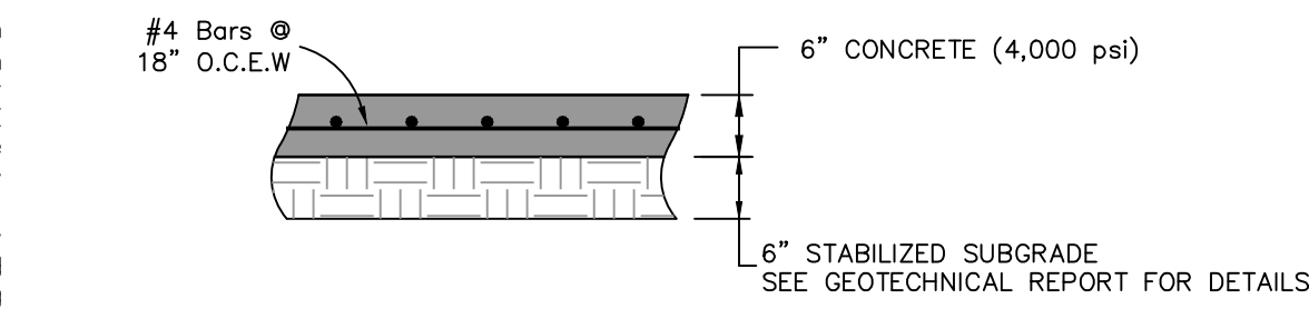
TYPICAL CONCRETE CROSS SECTION
